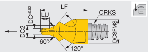
Fig. 2 Type B CRKS = Connection screw size
